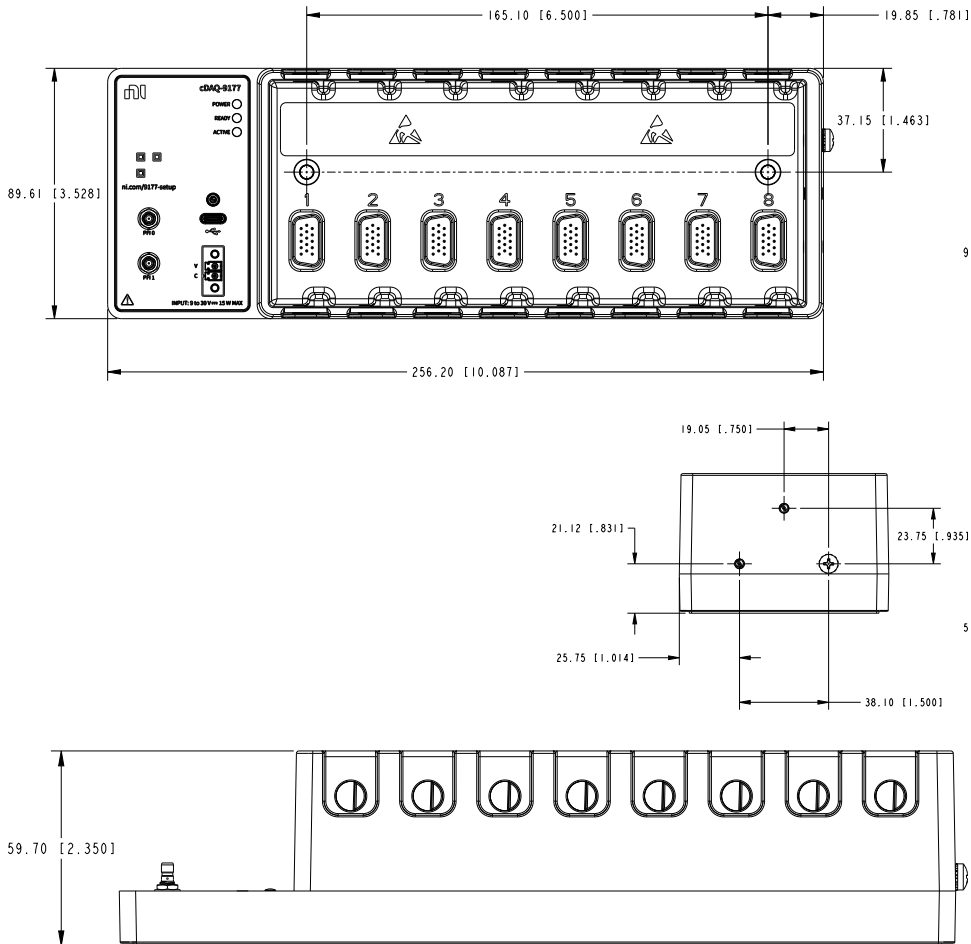
Figure 3. cDAQ-9177 Dimensions
